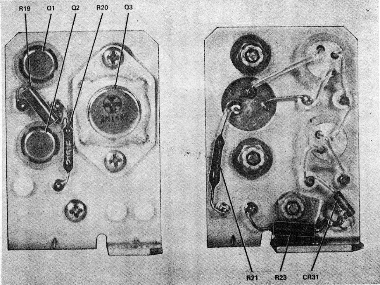
Figure 3-51. Power Supply PP-3518/PRC-47 (A8A5), Voltage Regulator Assembly TB1.
