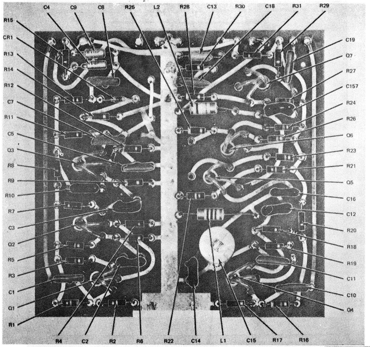
Figure 3-54. Oscillator Control C-4311/PRC-47 (A8A7), Card Assembly E1.
