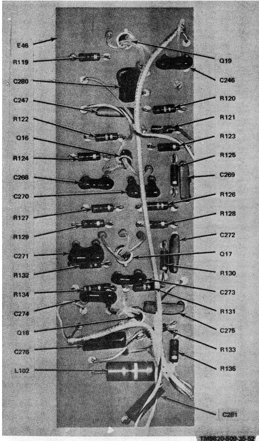
Figure 3-37. Signal Data Translator CV-1377A/PRC-47 (A8A3), Card Assembly E46.
