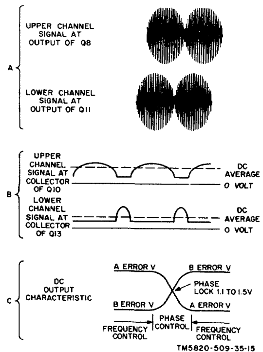
Figure 2 -15 Discriminator Circuit Waveforms.
