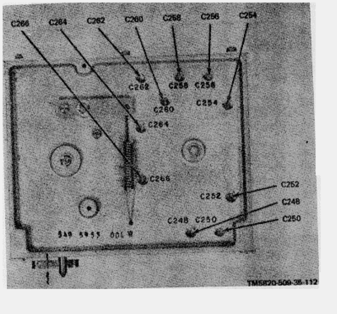
Figure 3-97. Signal Data Translator CV-1377A/PRC-47 (A8A3), Rear View, Location of Adjustments.
