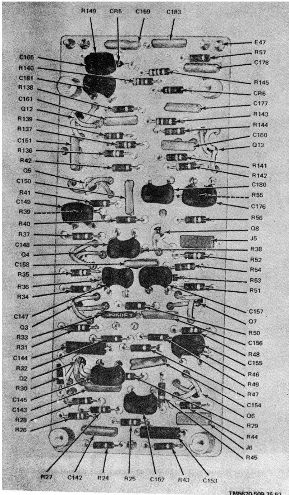
Figure 3-38. Signal Data Translator CV-1377/APC-47 (A8A3), Card Assembly E47.
